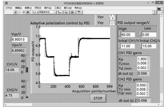
图 6 EOM 偏置在峰点时 PD 输出电压随期望值的变化曲线 Fig.6 Change curve of PD output voltage with the expected value when EOM biases at peak point
