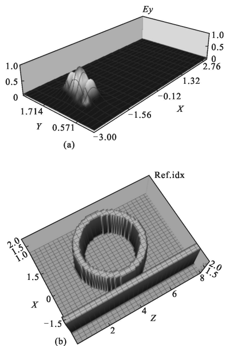
Fig.2 Input light plane, the refractive index distribution
