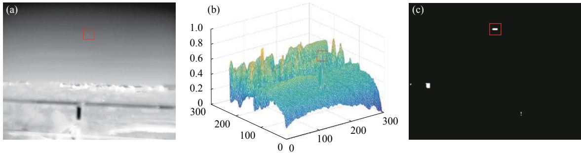
Fig.10 Detection result using only MRDLCM alone for Seq. 3. (a) The raw IR image sample of Seq. 3; (b) The MRDLCM result; (c) The threshold operation result on MRDLCM, more false alarms emerge
