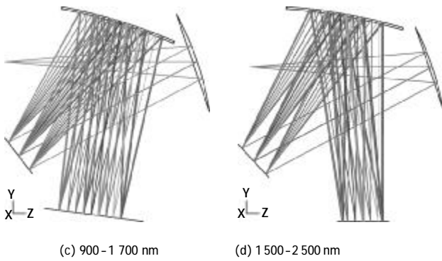
Fig.7 Light scattering system design
