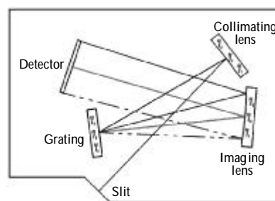
Fig.6 Crossed Czerny - Turner structure
