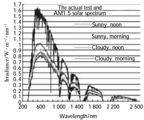
Fig.9 Solar spectrum curves with actual test
