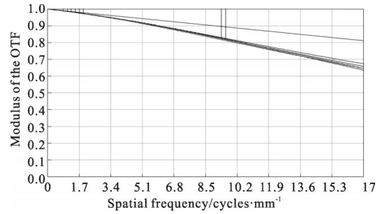
图 4 硫系玻璃与常用红外材料组合设计的系统 100^\circ\text{C} 时的 MTF Fig.4 MTF of system designed with chalcogenide glasses and common infrared materials at 100^\circ\text{C}
