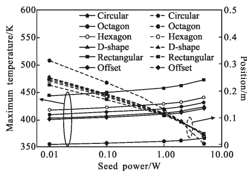
Fig.4 Seed powers versus maximum temperature (left) and positions with maximum temperature (right) for all kinds of DCFs
