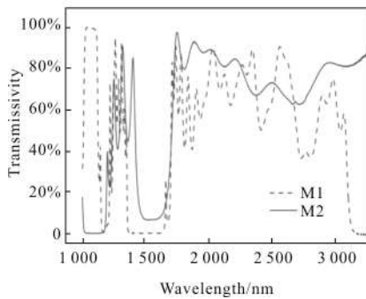
图 2 OPO 谐振腔镜 M1 和 M2 的透过率曲线 Fig.2 Transmissivity curves for the OPO cavity mirrors M1 and M2
