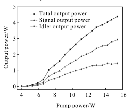
图 5 极化周期为 31 μm 时,输出功率与抽运功率关系曲线 Fig.5 Idler power, signal power and the total power versus the pump power at a grating period of 31 μm
