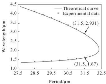
图 3 1 064 nm 激光作为基频光时的不同极化周期调谐的 MgO:PPLN 晶体的理论波长和实验波长图 Fig.3 Theoretical and experimental wavelengthes of different periods of MgO:PPLN crystal pumped by the fundamental laser at 1 064 nm
