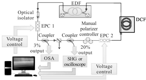
(a) 系统结构 (a) Experimental setup
