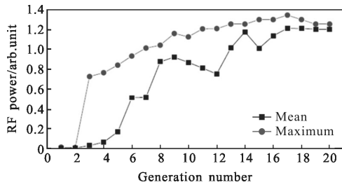
(b) 算法执行效果 (b) Effectiveness of the active control
