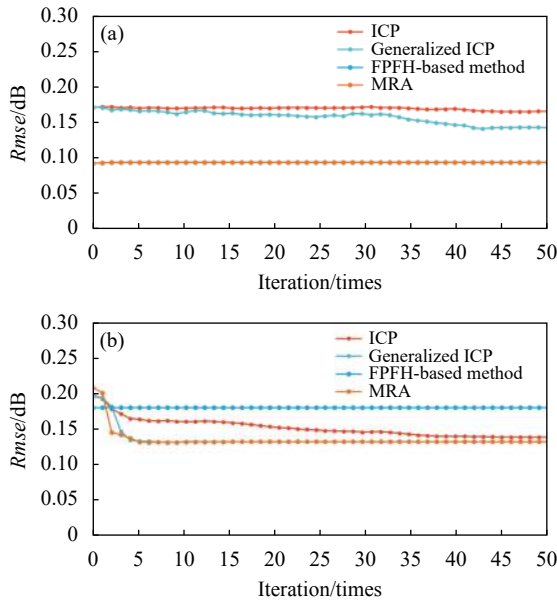
图 7 四种算法配准收敛曲线图。(a) 视角 37 和 38; (b) 视角 210 和 211 Fig.7 Convergence curves of four algorithms. (a) View 37 and 38; (b) View 210 and 211
