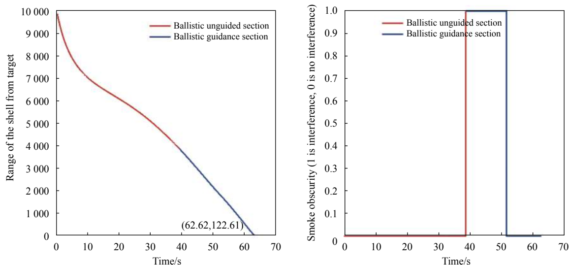
Fig.3 Distance curve and the interference result of the projectile with the initial velocity of 900 m/s and the ballistic deflection angle of 5^\circ
