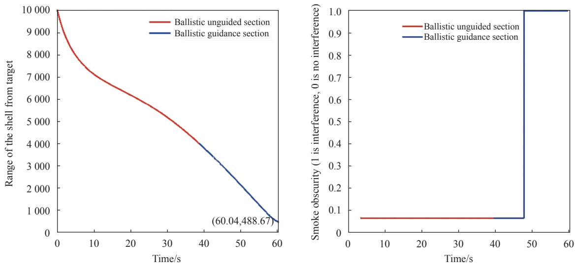
Fig.7 When the formation time of the smoke screen is 45 s, the distance curve of the projectile to the target and the interference situation
