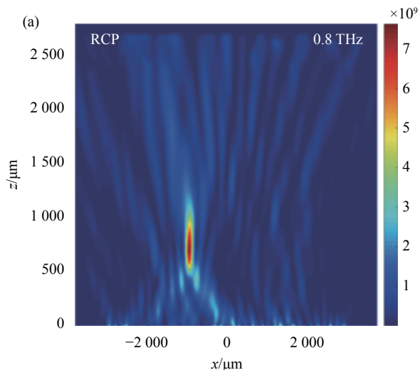
Fig.4 Intensity distribution of the focusing field when the RCP light incidence with the angle of 10^\circ (a) and 20^\circ (c), respectively; Intensity distribution of the focusing field when the LCP light incidence with the angle of 10^\circ (b) and 20^\circ (d), respectively
