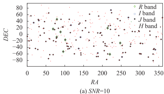
(a) SNR=10
